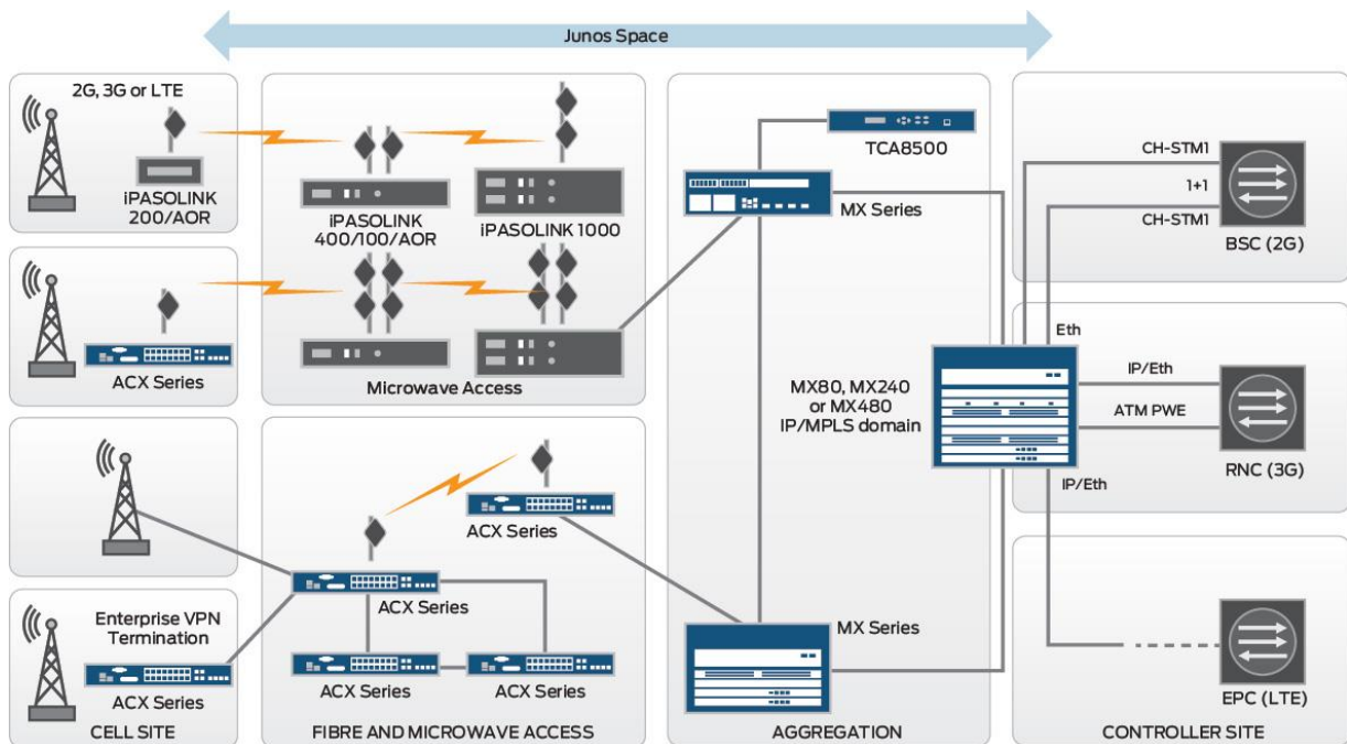
Figure 1: Expanded Juniper Networks & NEC macro and small cell universal backhaul
