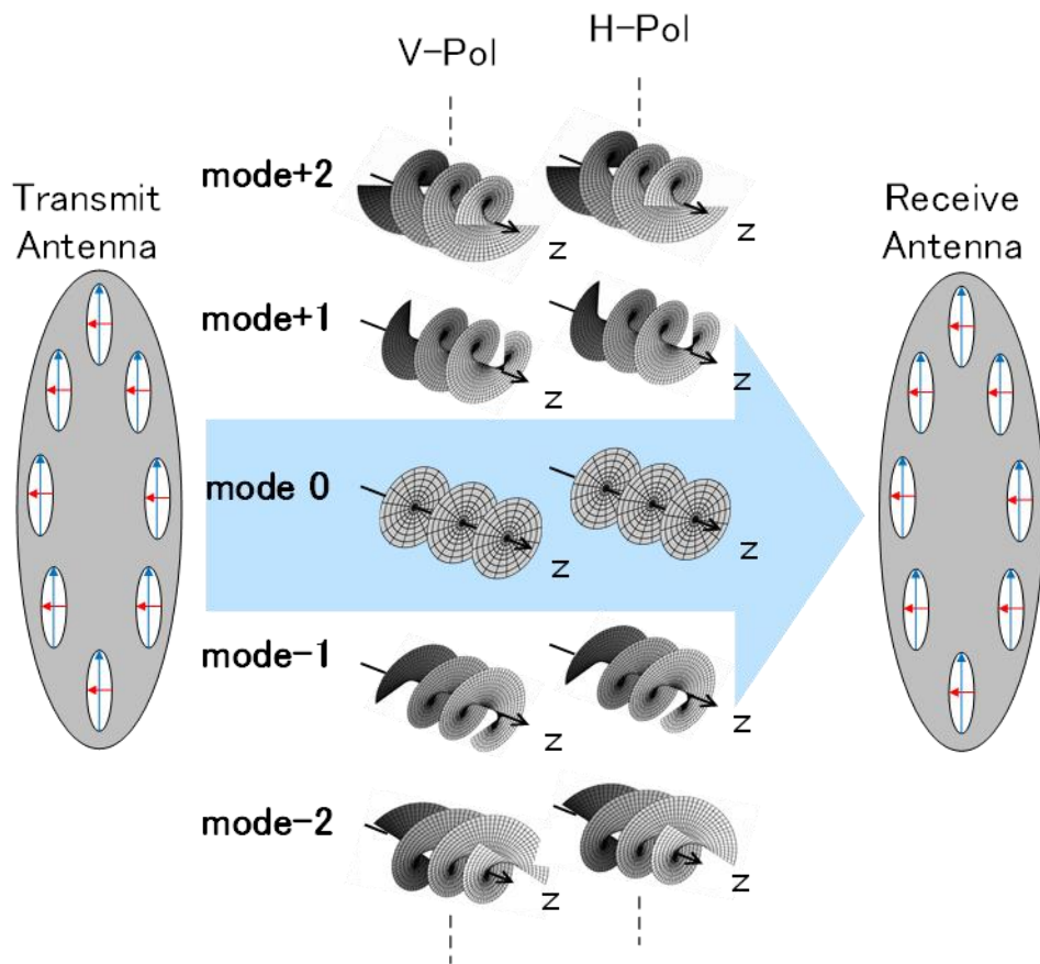
OAM mode and polarization multiplexing concept
