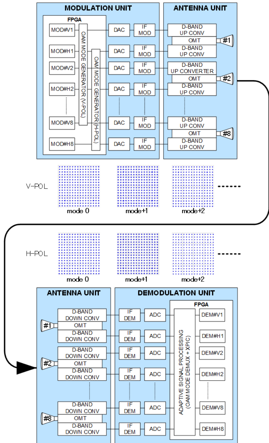
Block diagram of real-time digital wireless OAM mode multiplexing transmission equipment
