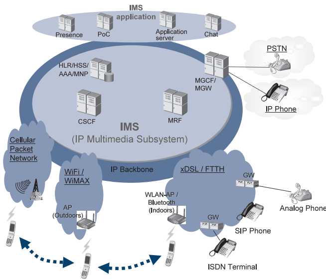
Fig. 2 FMC using IMS.
