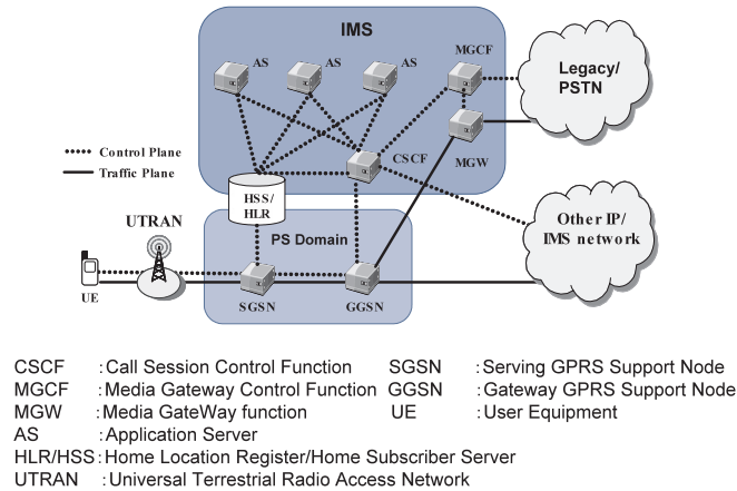
Fig. 1 IMS architecture.
