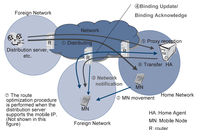
Fig. 3 Outline of Mobile IP operation.
