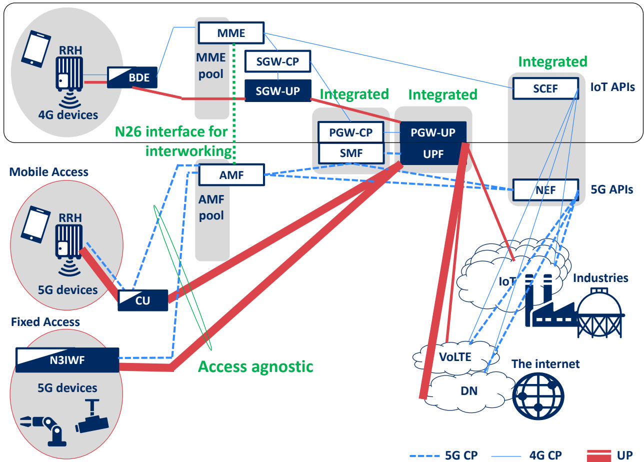
Figure 11: EPS – 5GS interworking deployment
