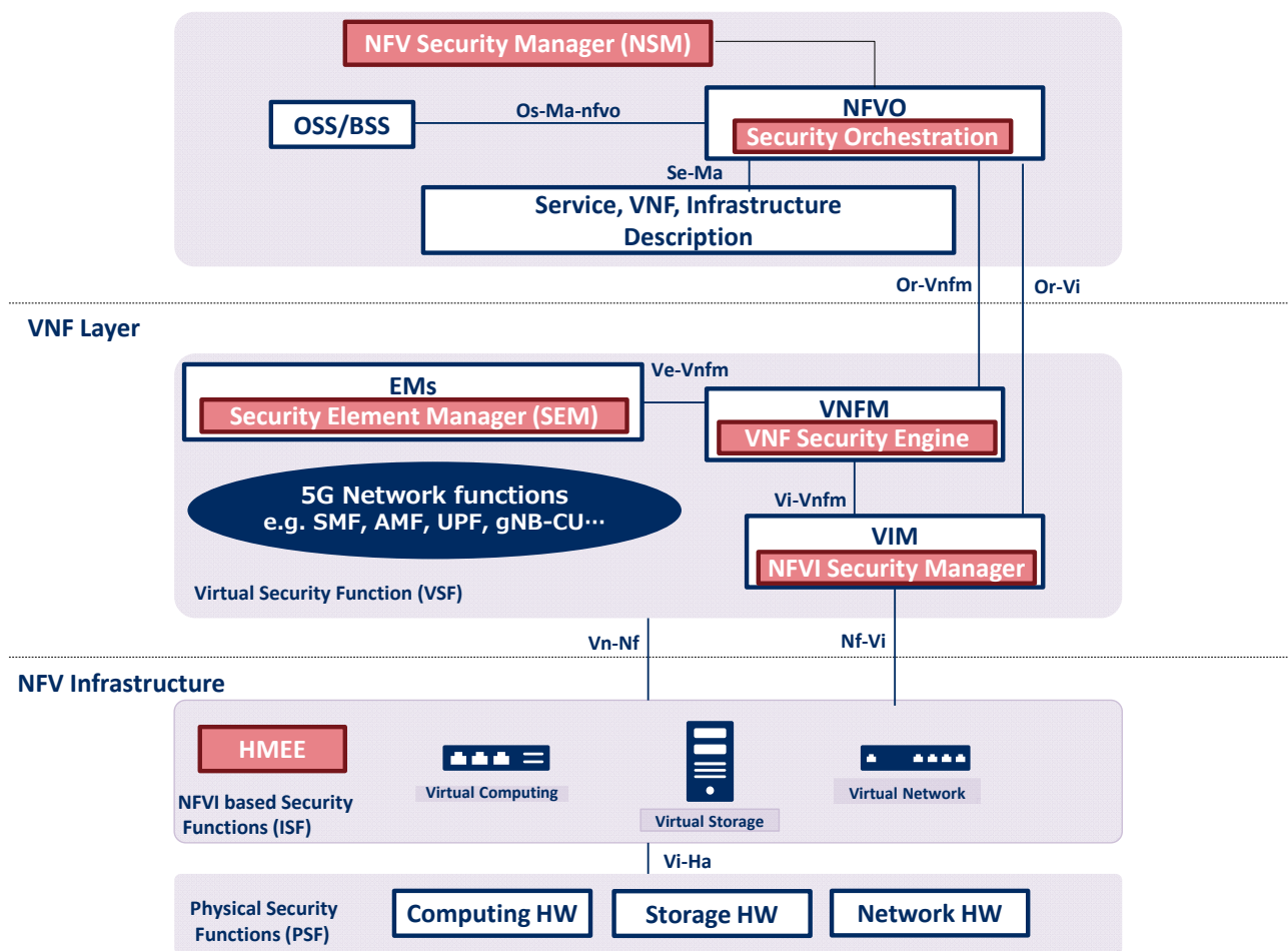
Figure 16: NFV Security logical representation
