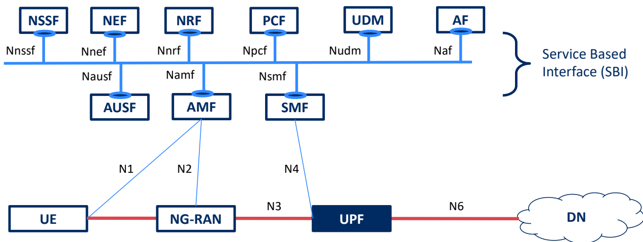
Figure 6: Service Based Architecture (SBA)
