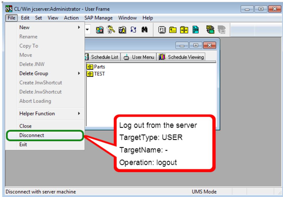
Figure 7.41. Logout Operation
