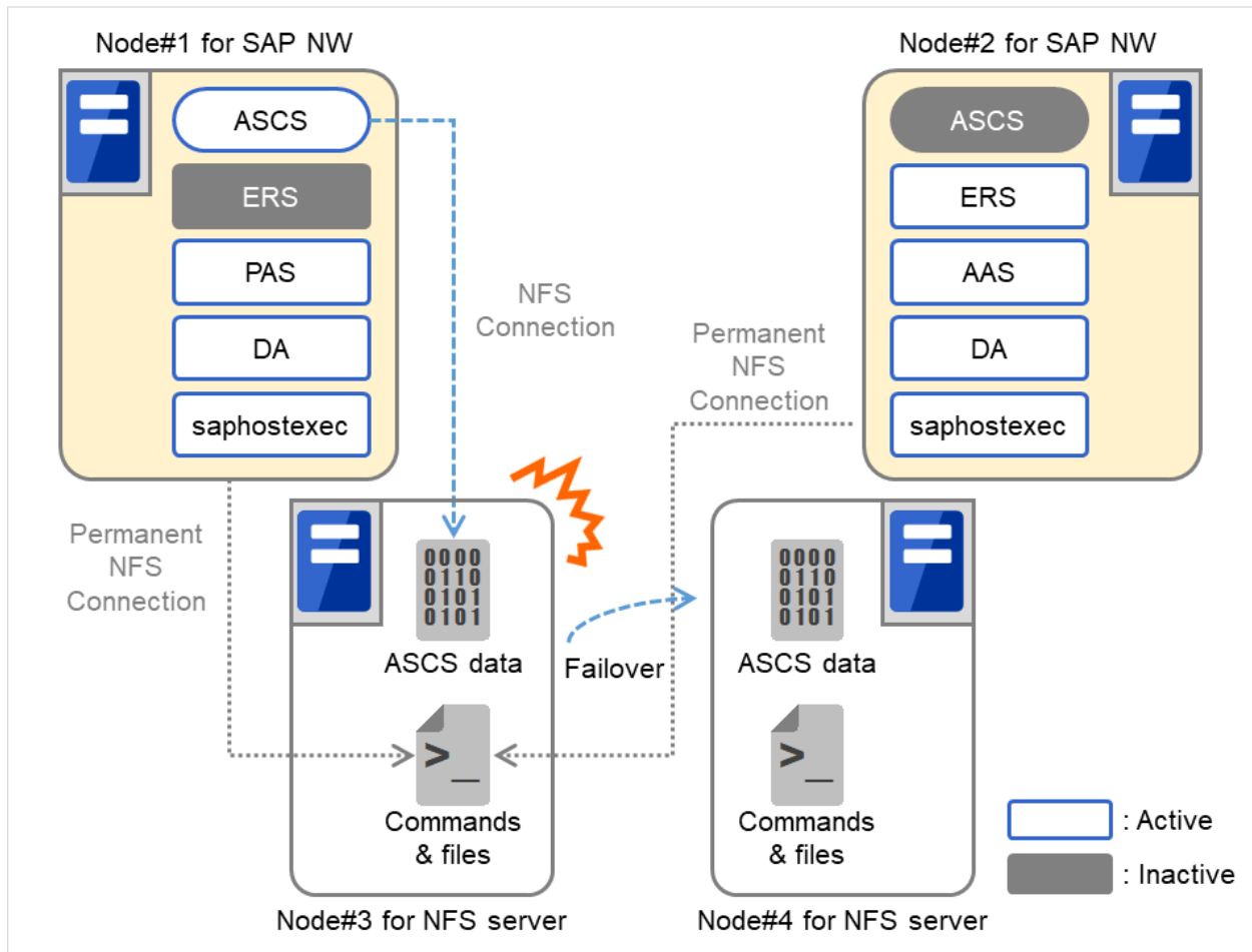
Fig. 3.5: System Configuration Using Two NFS Servers When a Failure Occurs in an NFS Server (1)
