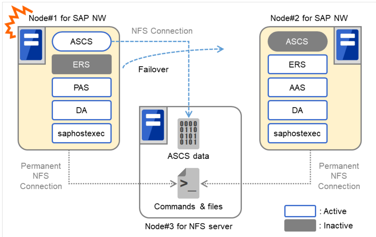
Fig. 3.1: System Configuration Using a Single NFS Server(1)
