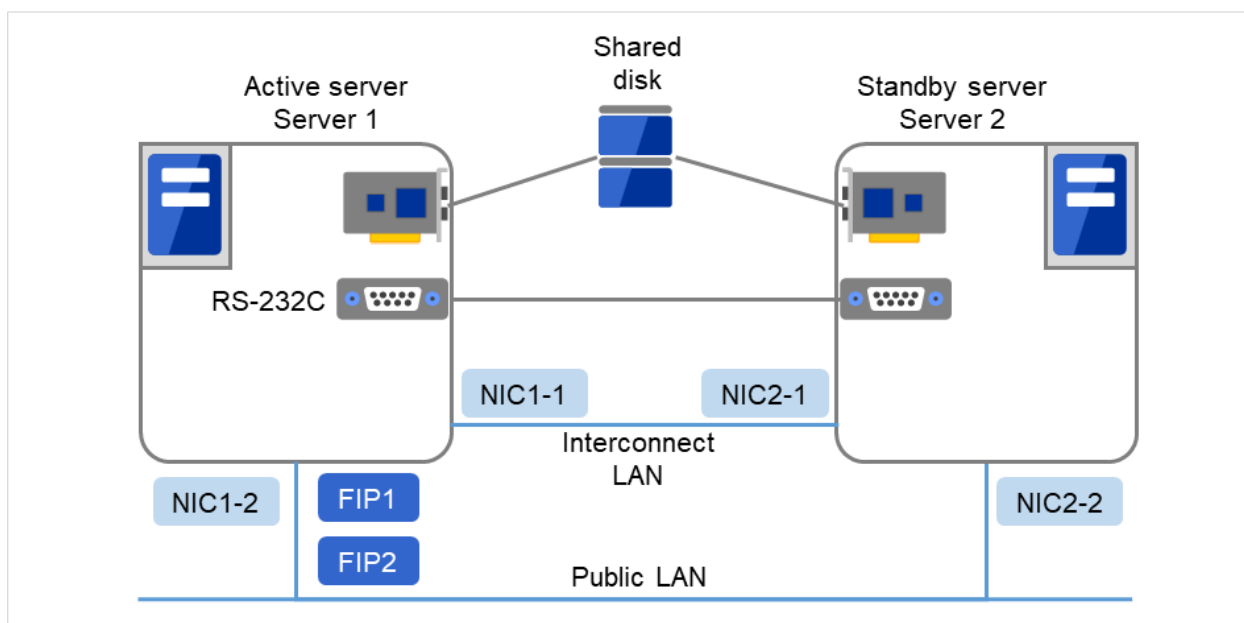
Fig. 3.7: Example of cluster configuration (Shared disk type)
