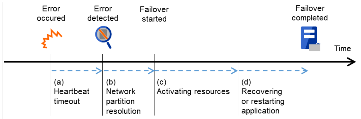
Fig. 3.6: Failover time chart
