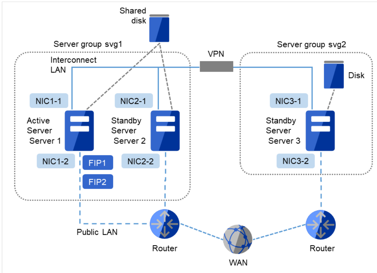
Fig. 3.11: Example of cluster configuration (Hybrid disk type, remote cluster)
