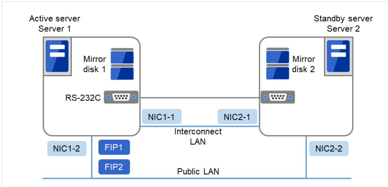
Fig. 3.8: Example of cluster configuration (1) (Mirror disk type)
