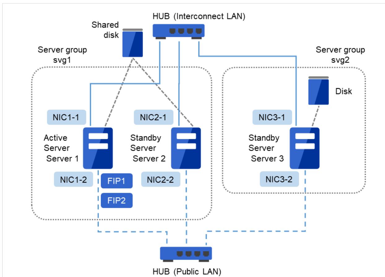
Fig. 3.10: Example of cluster configuration (Hybrid disk type)
