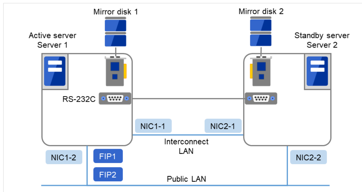
Fig. 3.9: Example of cluster configuration (2) (Mirror disk type)
