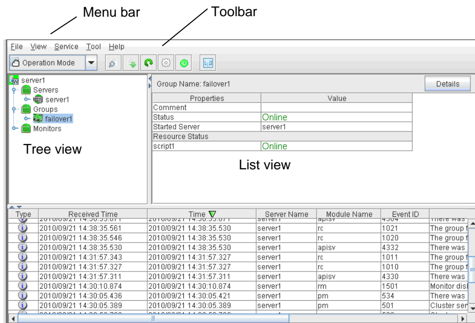
Alert view
