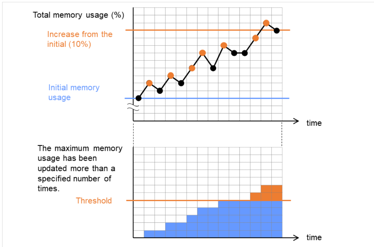
Fig. 6.28: The maximum value of the memory usage is updated more than the specified number of times, and the memory usage increases by more than 10% from its initial value (an error detected)
