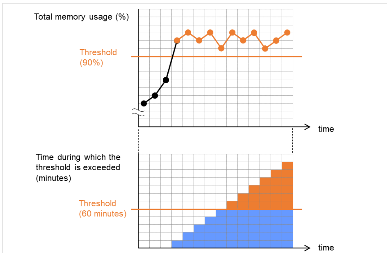
Fig. 6.22: The total memory usage remains at the total memory usage threshold or higher for a certain duration of time
