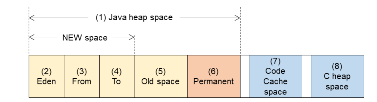
Fig. 6.19: Java VM memory space (Oracle Java 7)
