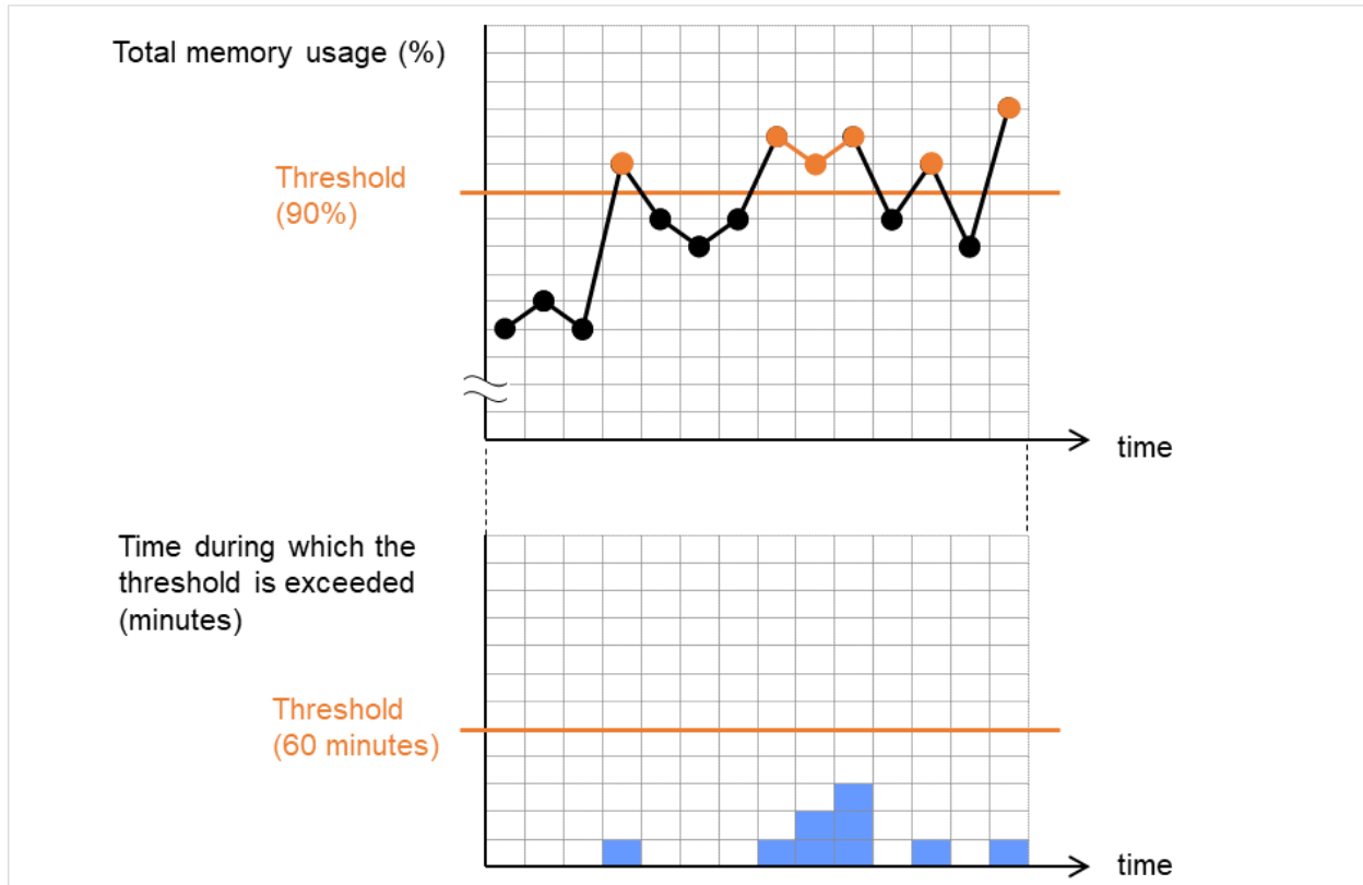
Fig. 6.23: The state of exceeding the total memory usage threshold does not persist for a certain duration of time (no error detected)
