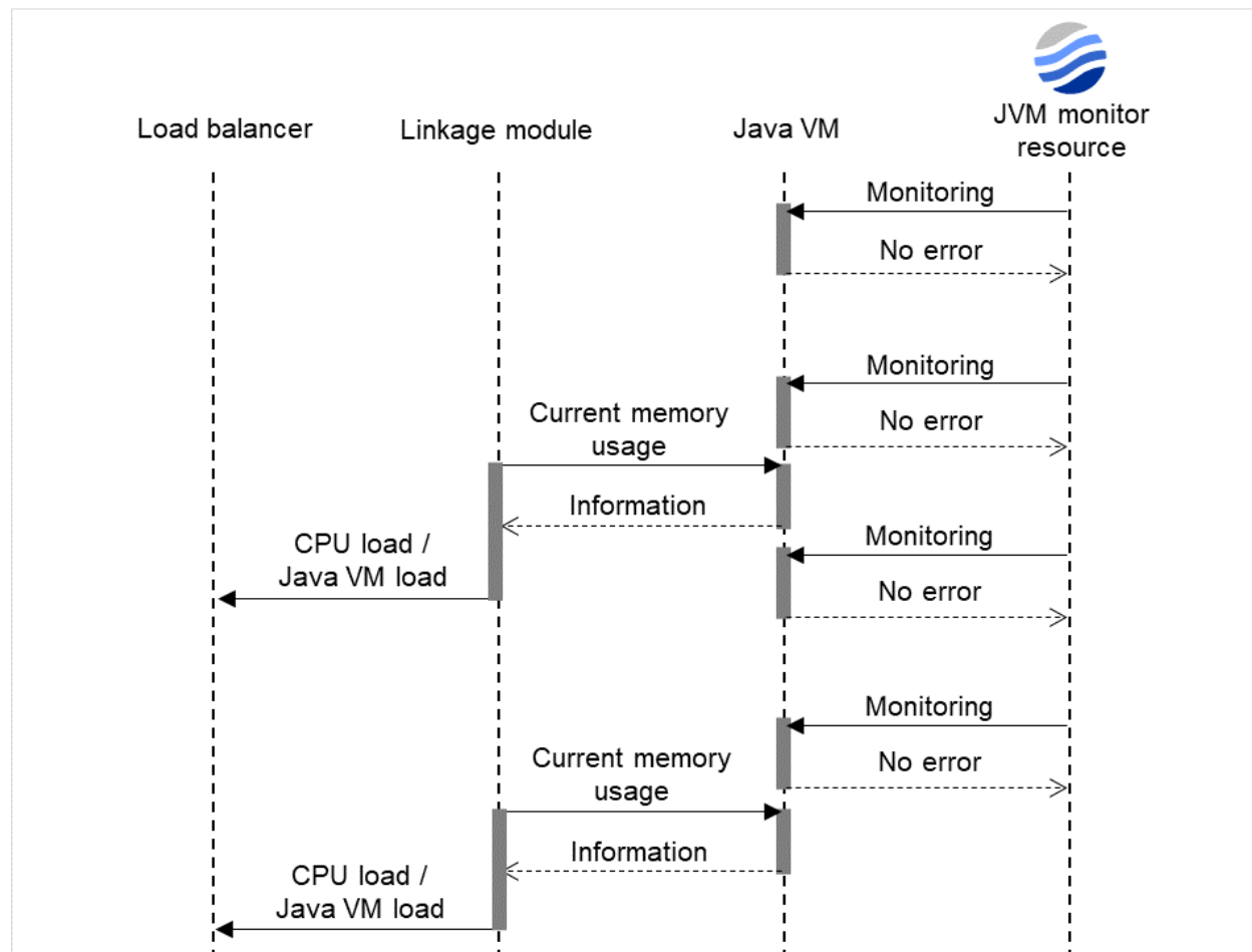
Fig. 6.18: Settings of the load calculation function
