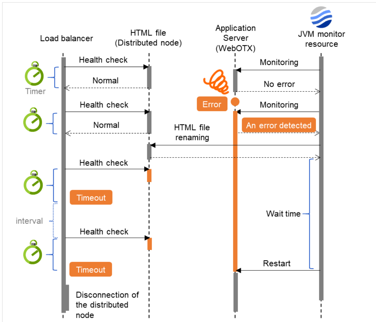
Fig. 6.15: JVM monitor resource health check function for the load balancer
