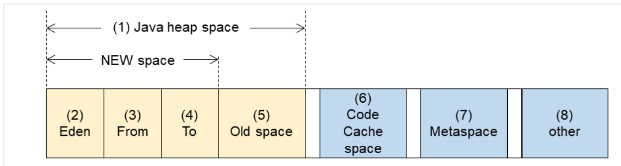
Fig. 6.20: Java VM memory space (Oracle Java 8/Oracle Java 9/Oracle Java 11)
