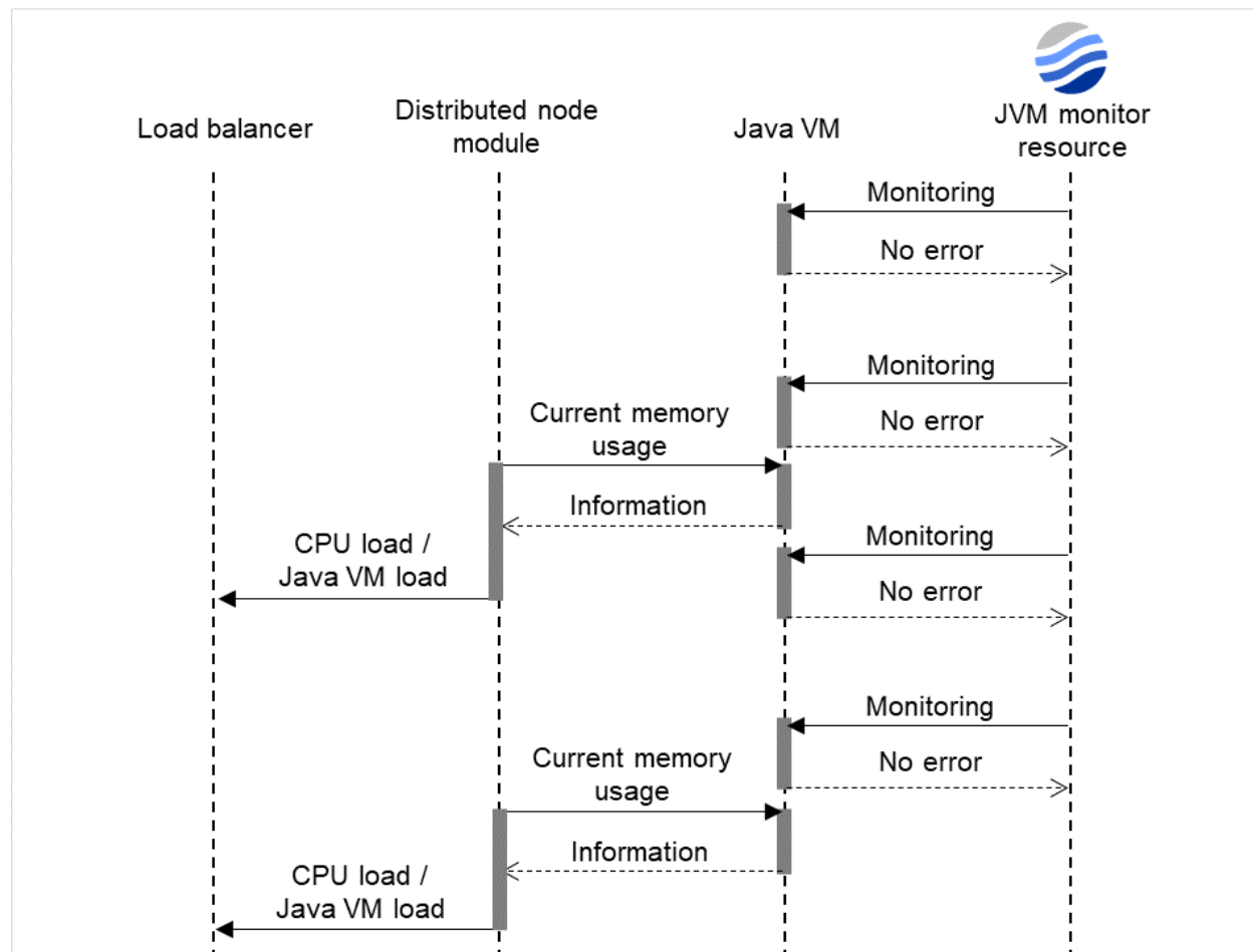
Fig. 6.16: Load calculation function for the distributed node module
