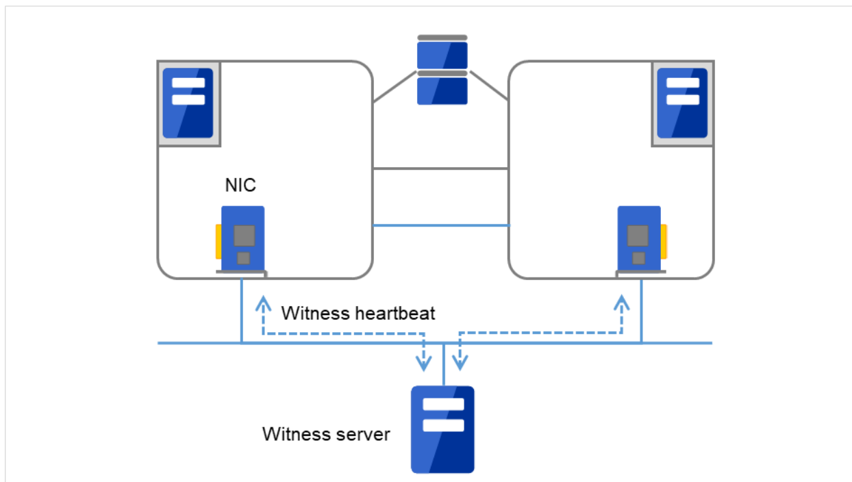
Fig. 3.33: Witness heartbeat
