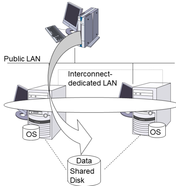
Fig. 3.4: System configuration
