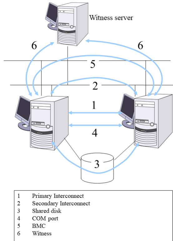
Fig. 3.2: Server monitoring
