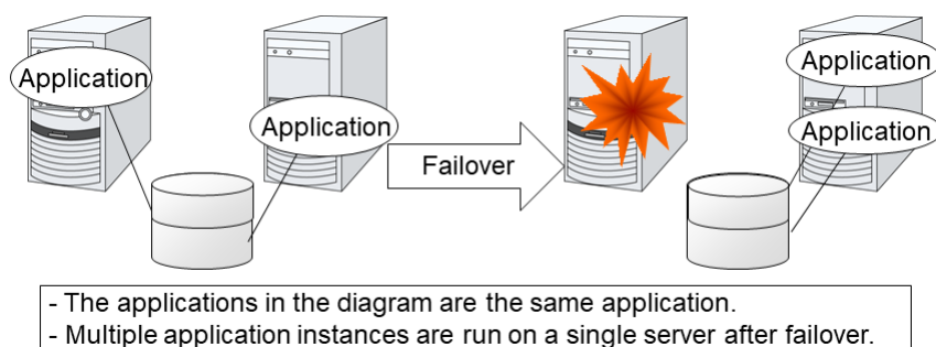
Fig. 3.6: Same application multi directional standby cluster system
