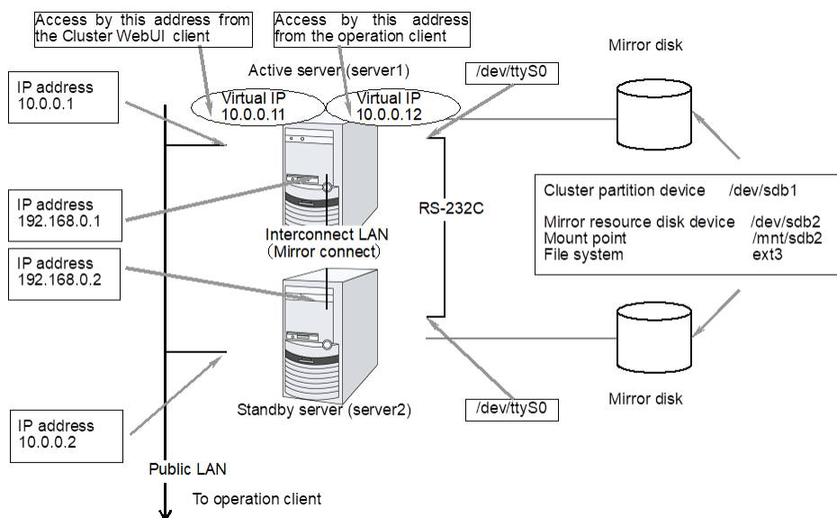
Fig. 3.11: Sample of cluster environment when mirror disks are used (when disks for cluster partition and data partition are prepared)
