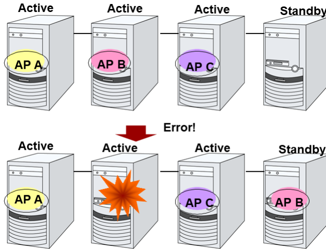
Fig. 3.8: Node to Node configuration
