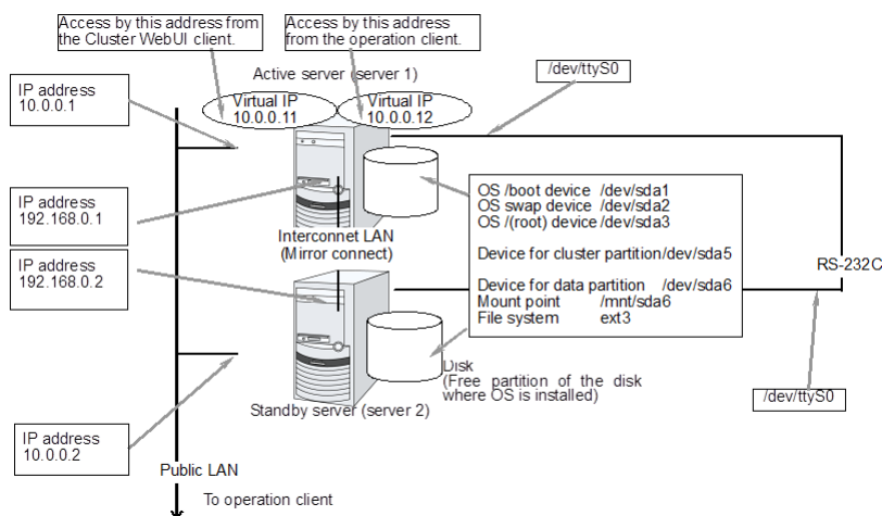
Fig. 3.10: Sample of cluster environment when mirror disks are used (when allocating cluster partition and data partition to the disk where OS is installed)
