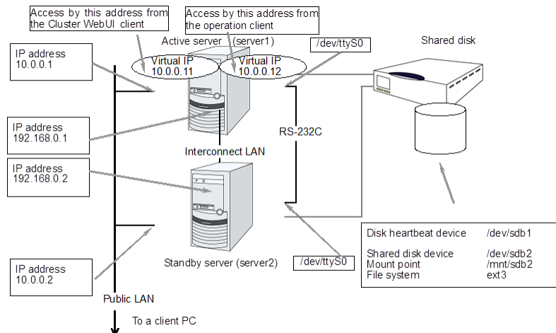
Fig. 3.9: Sample of cluster environment when a shared disk is used
