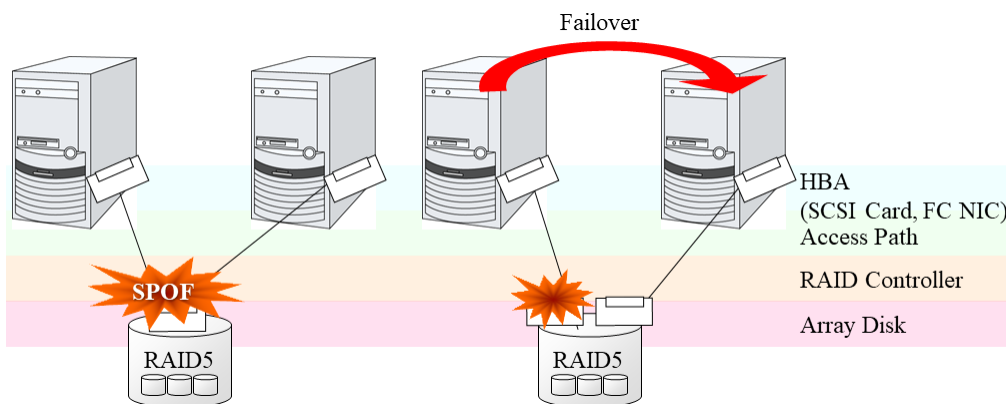
Fig. 2.9: Example of the shared disk RAID controller and access paths being SPOF (left) and an access path connected to a RAID controller
