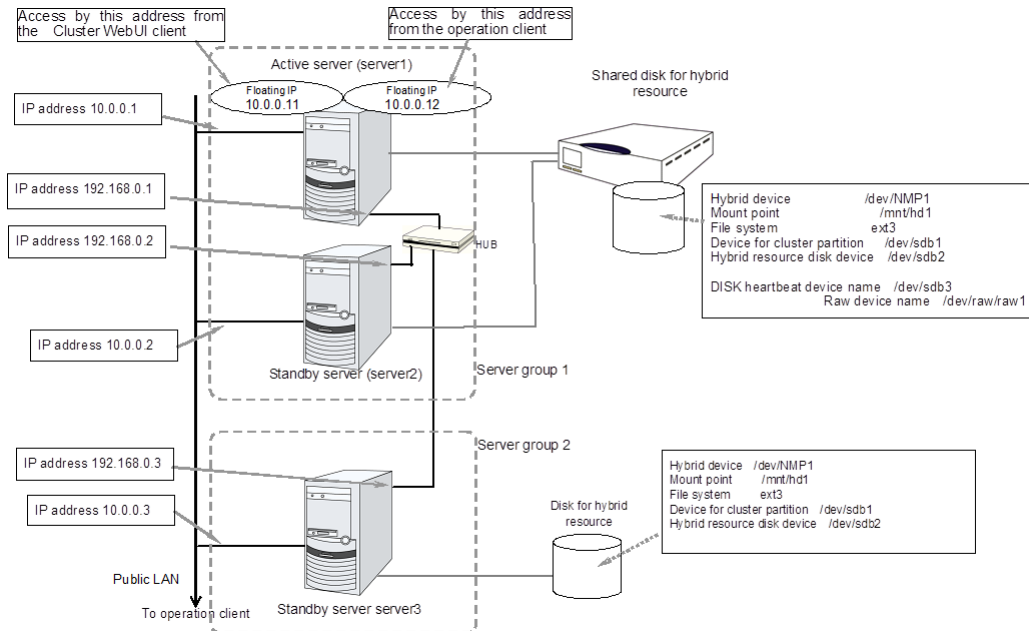
Fig. 3.12: Sample of cluster environment where hybrid disks are used (two servers use a shared disk and the third server's general disk are used for mirroring)
