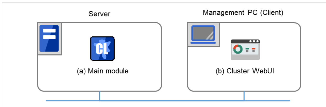
Fig. 2.3: Software configuration
