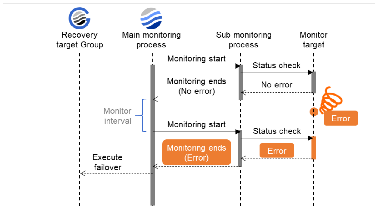
Fig. 7.3: Monitoring interval (an error detected, without monitor retry settings)
