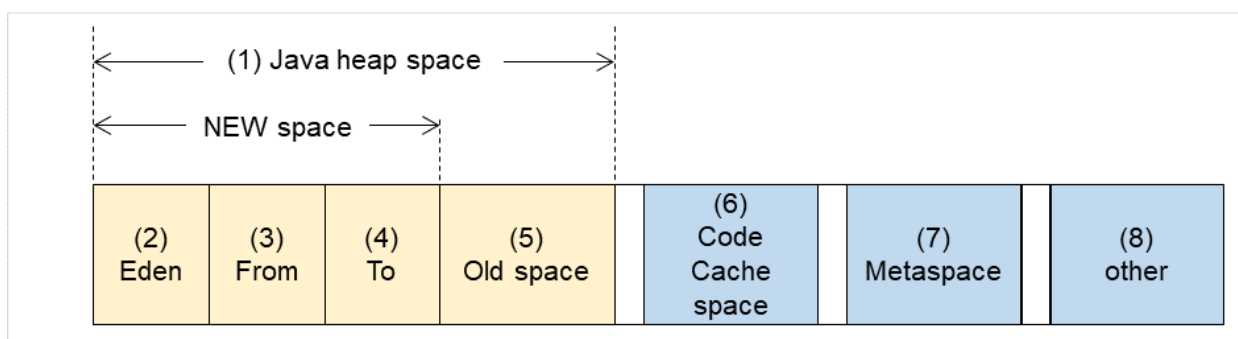
Fig. 5.10: Java VM memory space (Oracle Java 8/Oracle Java 9/Oracle Java 11)
