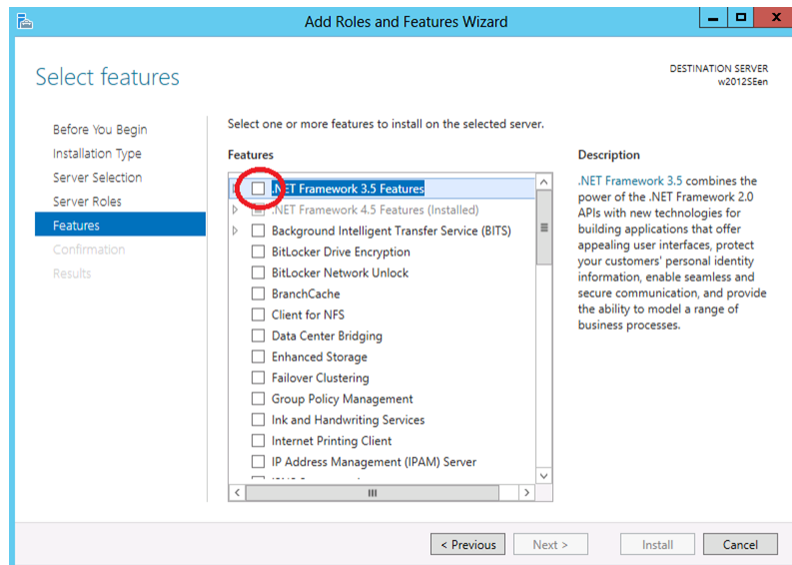
Fig. 2.8: Select Features
