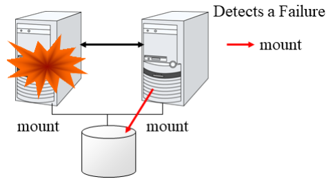
Fig. 2.11: Inheriting data
