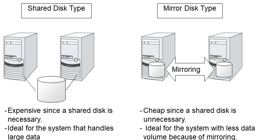
Fig. 2.1: HA cluster configuration
