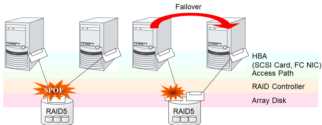
Fig. 2.13: Example of the shared disk RAID controller and access paths being SPOF (left) and an access path connected to a RAID controller
