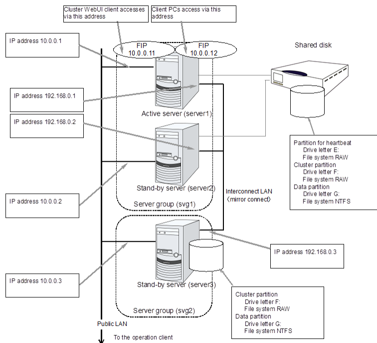
Fig. 3.7: Sample of the hybrid disk type cluster environment
