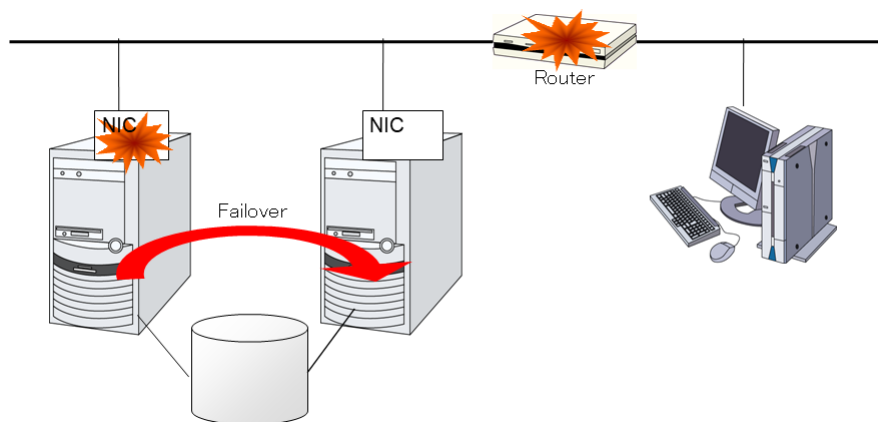
Fig. 2.15: Example of router becoming SPOF
