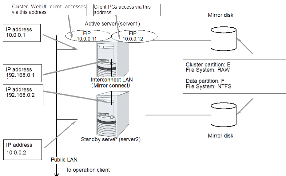
Fig. 3.6: Sample of cluster environment when mirror disks are used (in case of preparing disks for cluster partition and data partition)
