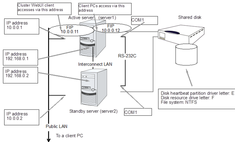
Fig. 3.4: Sample of a cluster environment when a shared disk is used
