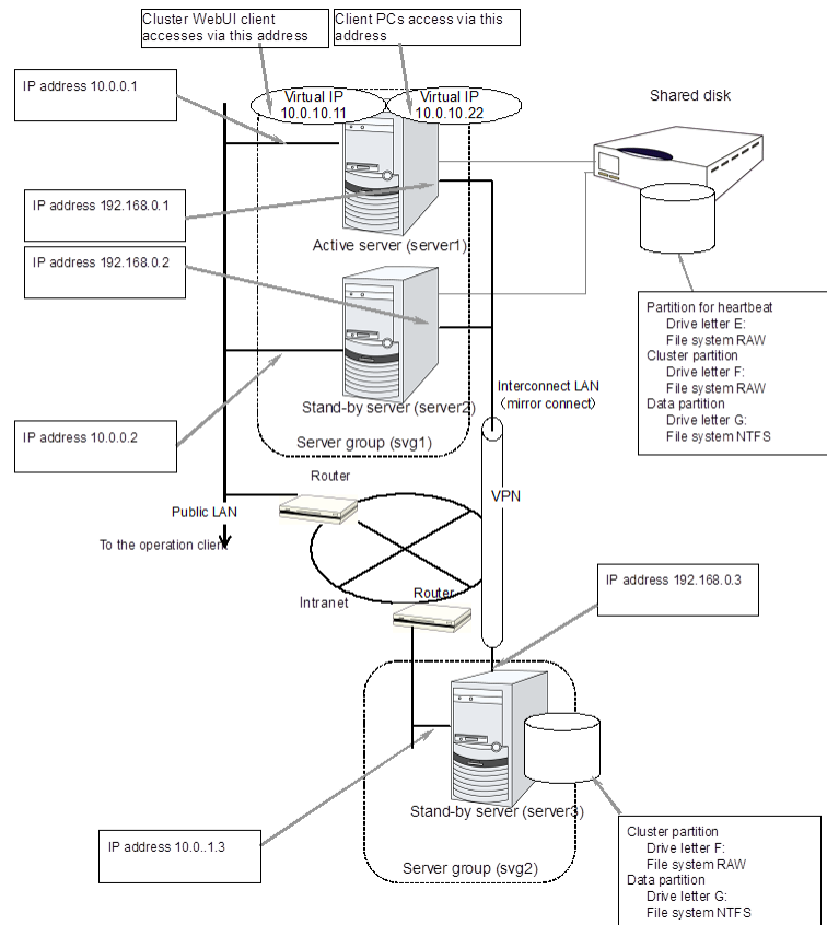
Fig. 3.8: Sample of the remote cluster environment when the hybrid disk is used
