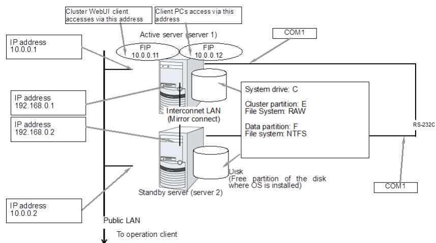
Fig. 3.5: Sample of a cluster environment when mirror disks are used (when allocating cluster partition and data partition on the disk where OS is installed)
