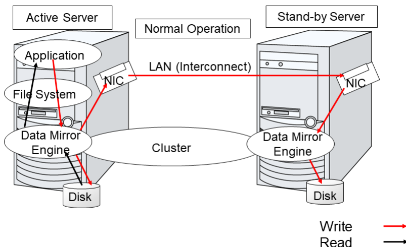
Fig. 2.4: Data mirror mechanism
