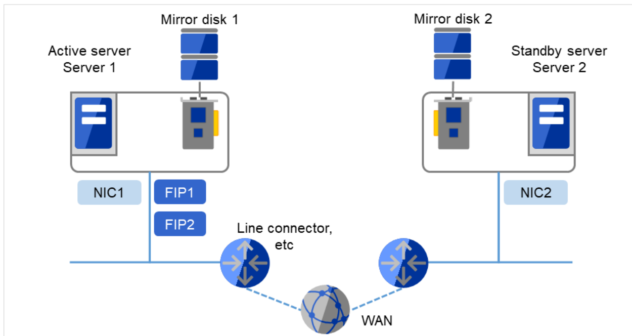
Fig. 6.4: Example of a 2-node cluster with a remote configuration using mirror disk resources
