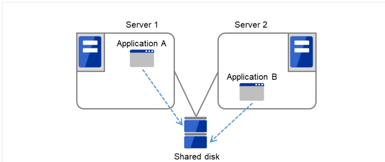
Fig. 3.12: Multi-directional standby cluster system with different applications (1)
