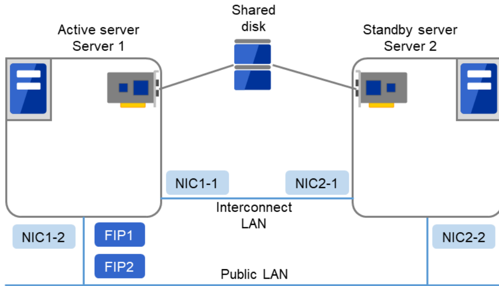
Fig. 3.16: Example of cluster configuration (Shared disk type)
