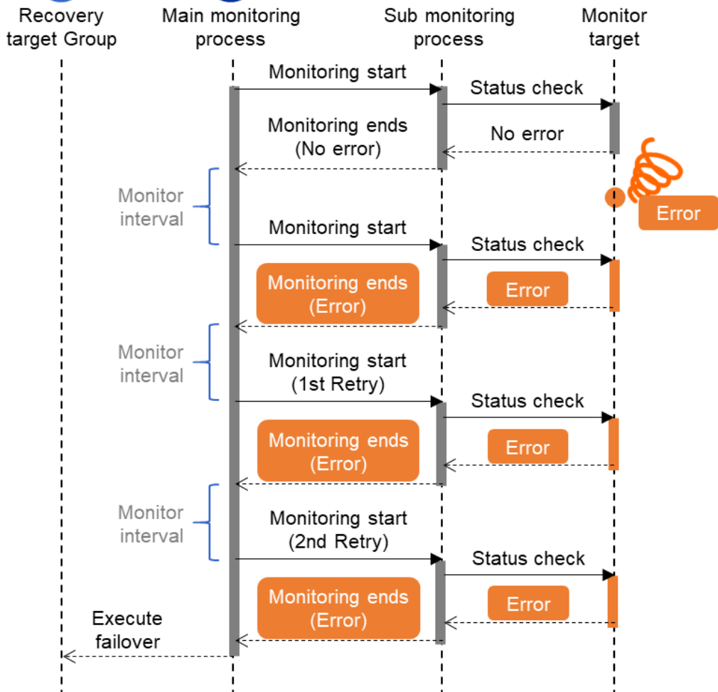
Fig. 4.4: Monitor interval (when an error is detected with monitor retry setting)
