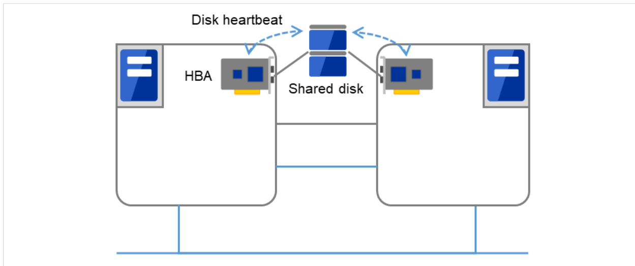
Fig. 5.3: Disk heartbeat
