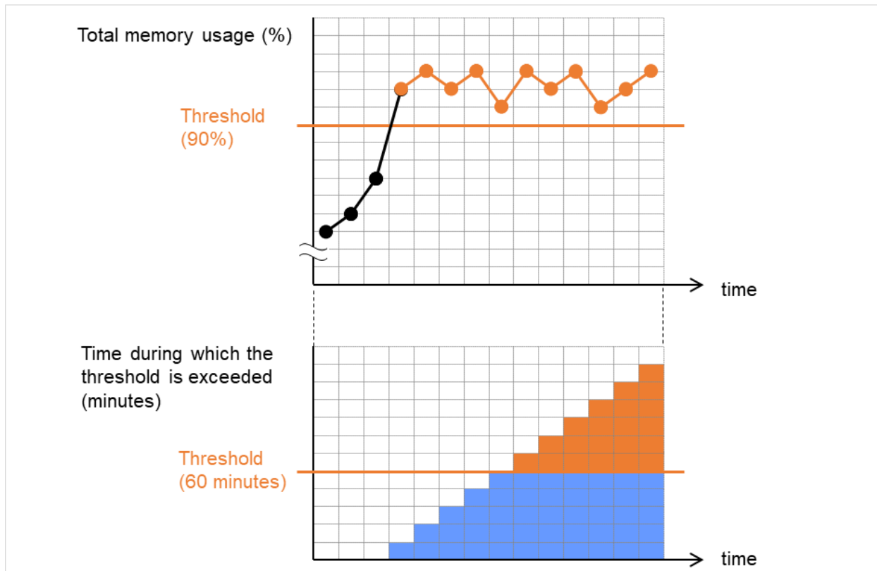
Fig. 6.18: The total memory usage remains at the total memory usage threshold or higher for a certain duration of time
