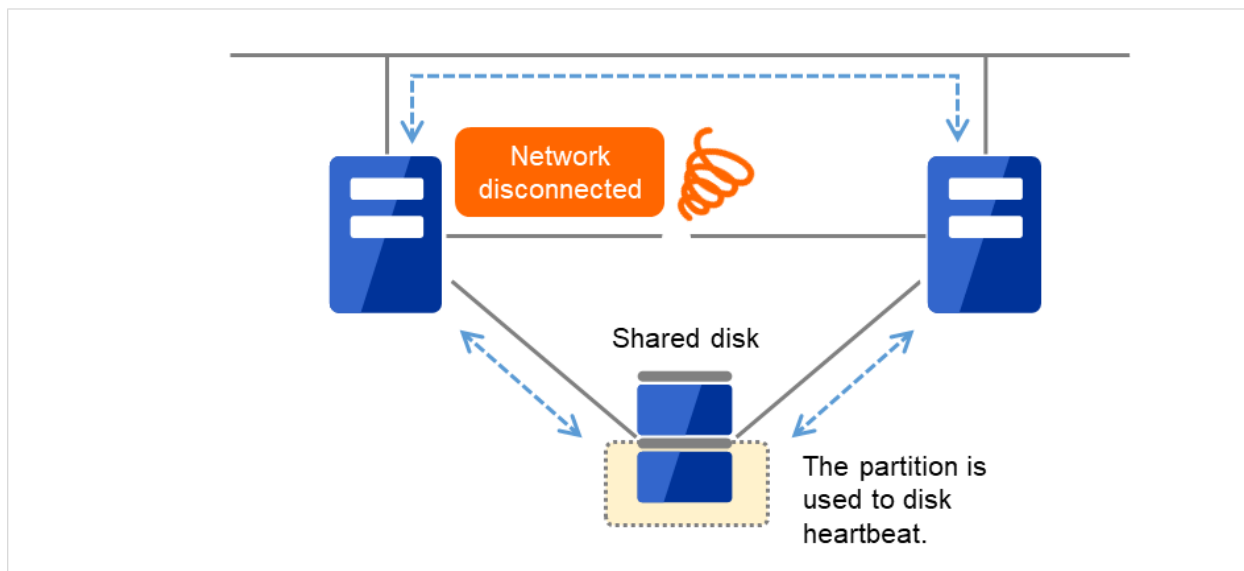
Fig. 5.6: Disk heartbeat resource (2)
