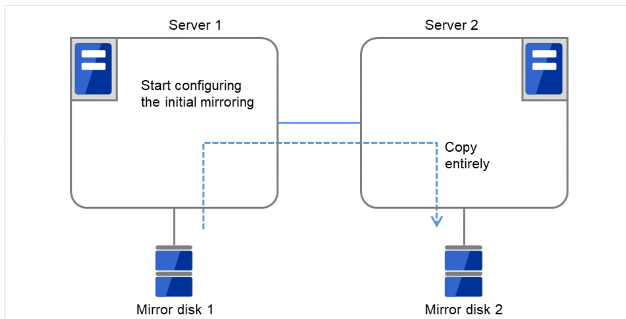
Fig. 3.100: Example of mirror disk construction: executing only initial mirror construction (2)
