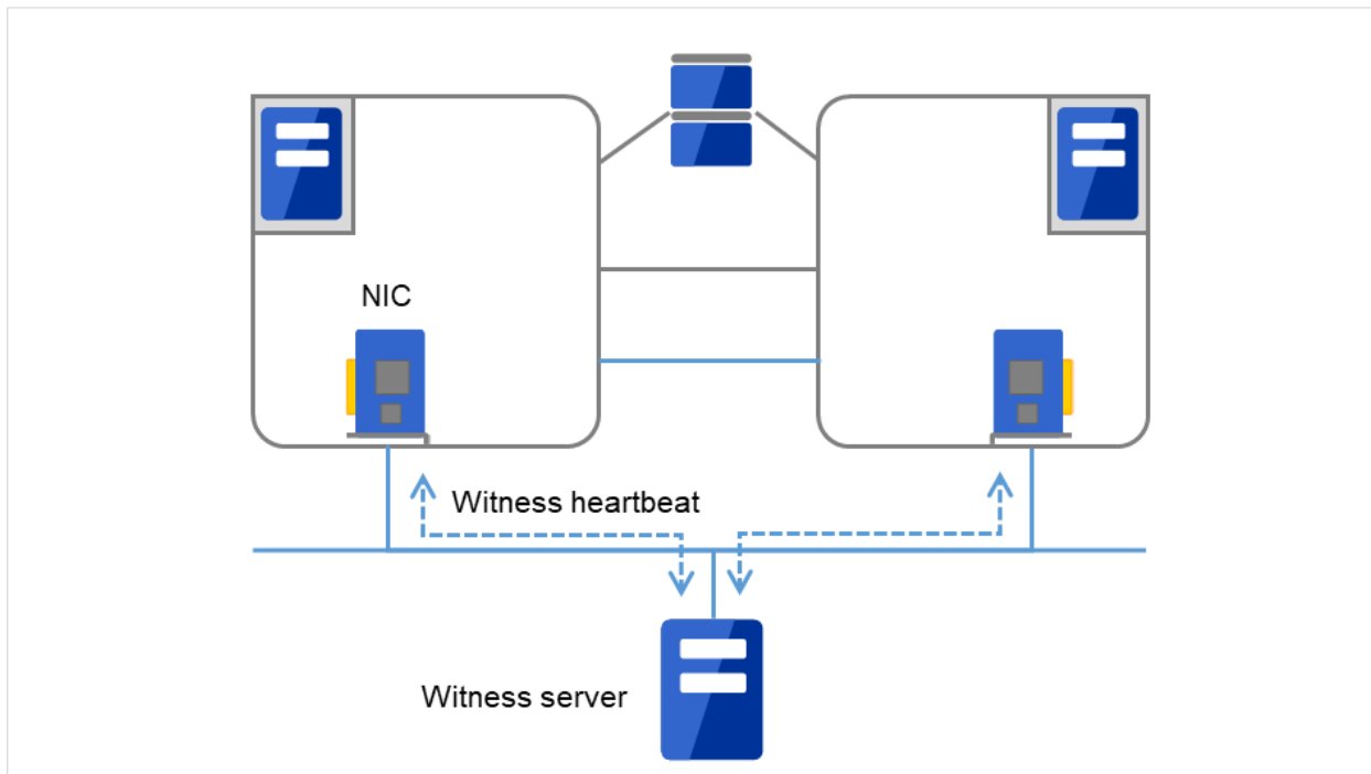
Fig. 5.4: Witness heartbeat
