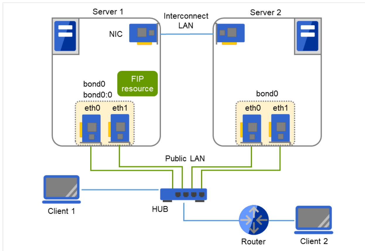
Fig. 8.6: An example of the floating IP resource on bonding
