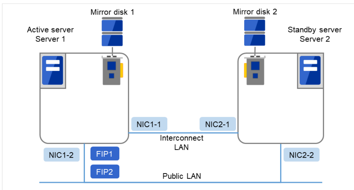
Fig. 6.3: Example of a 2-node cluster with mirror disk resources
