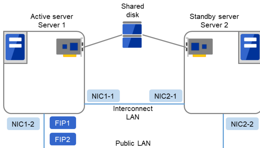
Fig. 6.2: Example of a 2-node cluster with a disk resource
