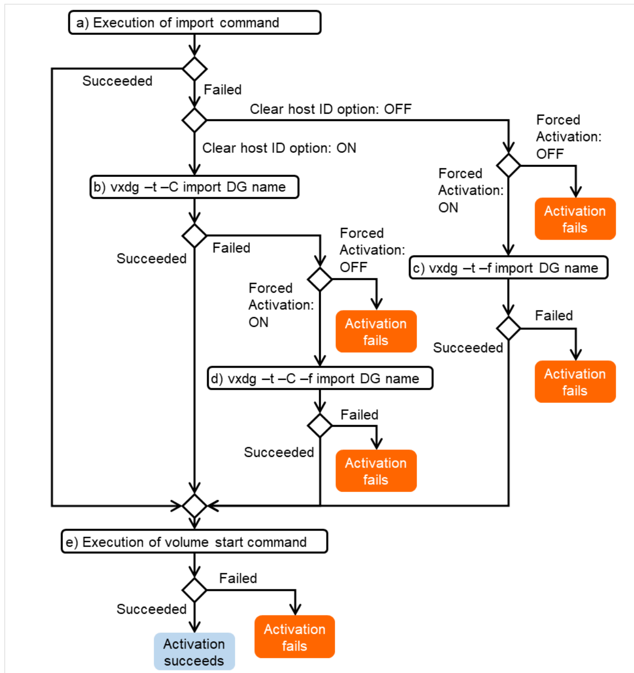
Fig. 3.126: Resource activation sequence (vxvm)
