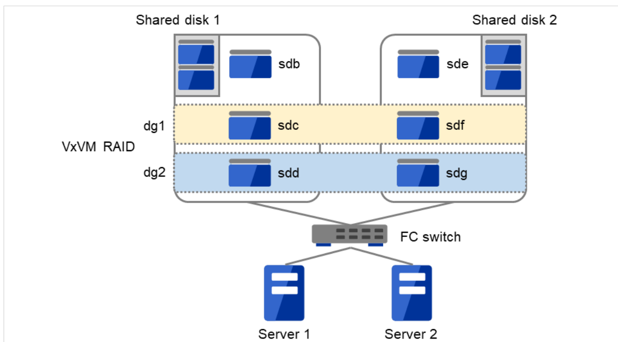
Fig. 6.6: Configuration of VERITAS Volume Manager supported by EXPRESSCLUSTER
