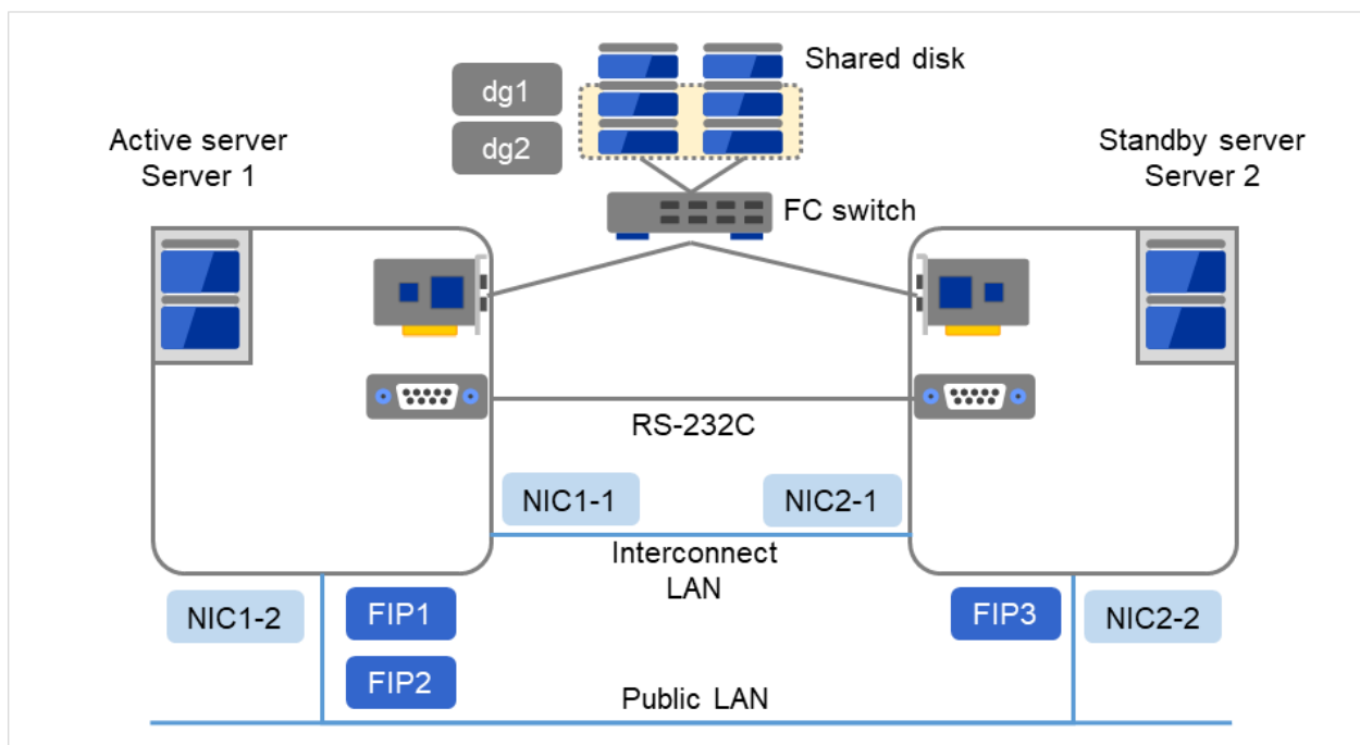
Fig. 6.7: Example of a 2-node cluster with VxVM
