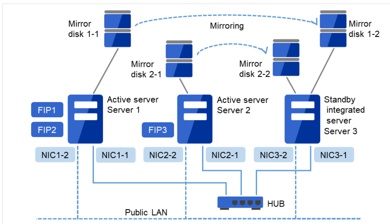
Fig. 6.8: Example of a 3-node cluster with mirror disks
