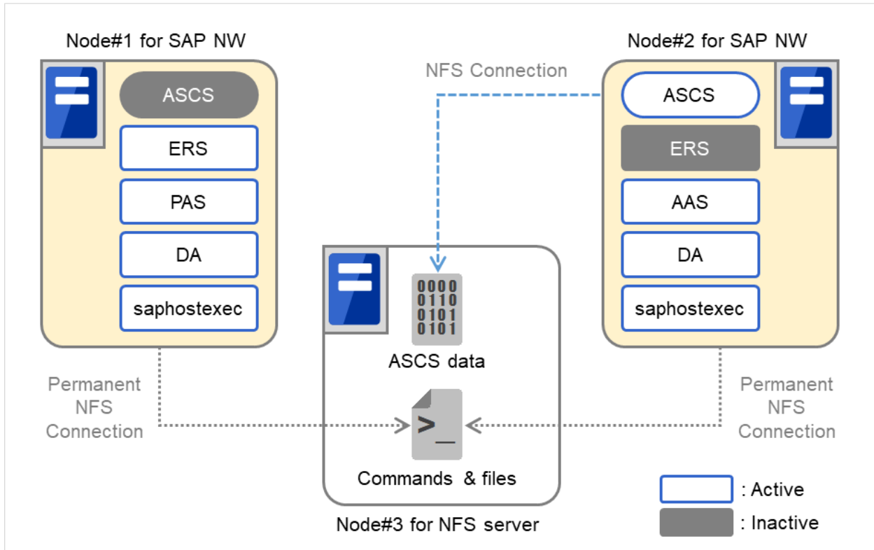
Fig. 3.2: System Configuration Using a Single NFS Server(2)
