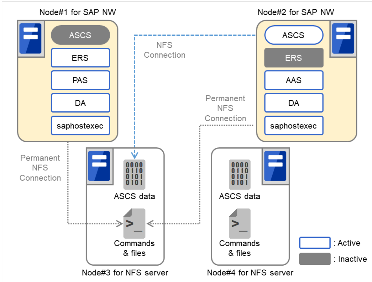
Fig. 3.4: System Configuration Using Two NFS Servers When a Failure Occurs in an SAP NW Server (2)
