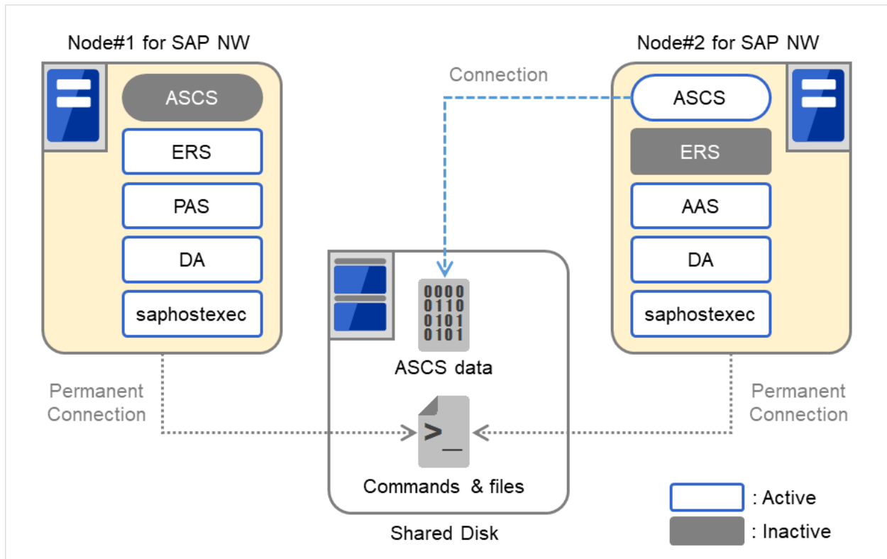
Fig. 2.2: Configuration diagram (with ENSA used) (2)
