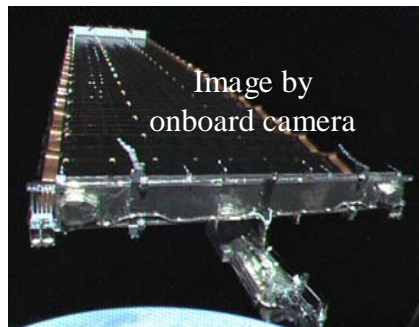
COMETS (1997) GaAs Flexible Solar Array 3m x 15m
