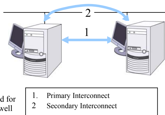
Figure 2-2: Server monitoring
