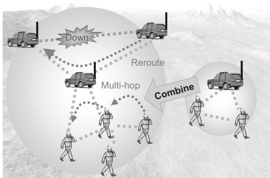
Fig. 2 Ad-hoc network.
