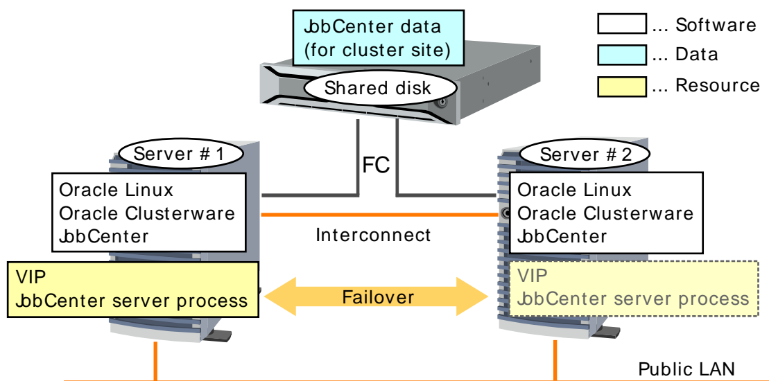
Figure 7.1. Configuration Example
