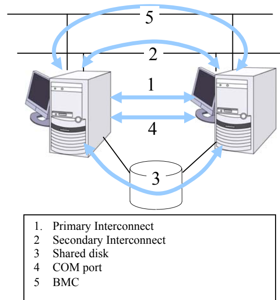
Figure 2-2 Server monitoring
