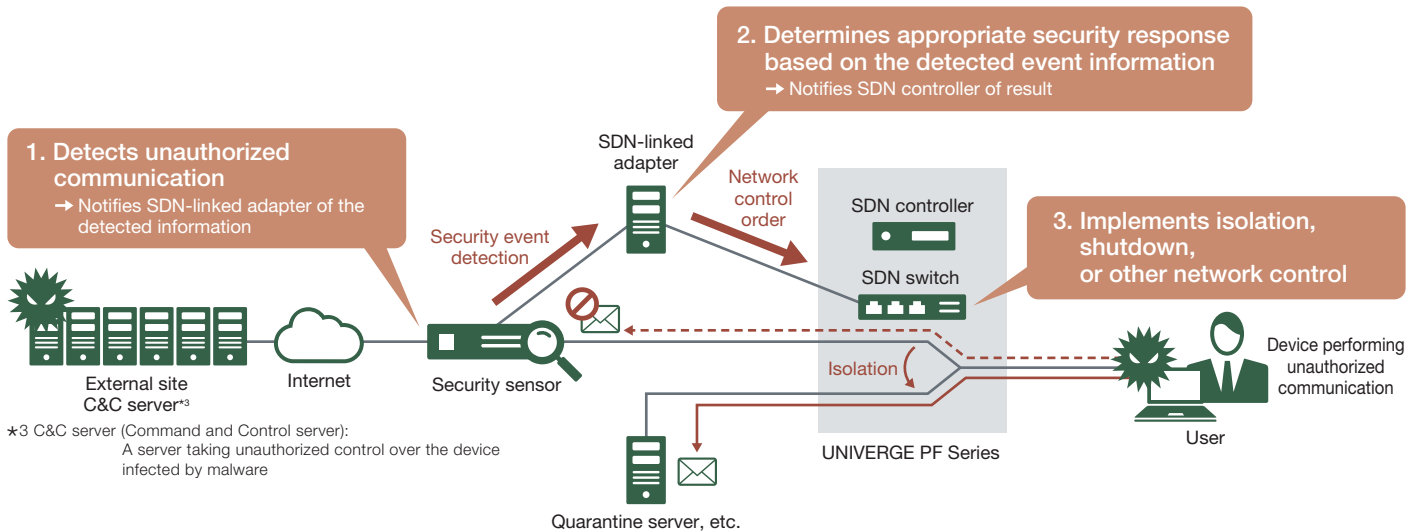
SDN-linked Cyber Attack Automated Defense Solution
