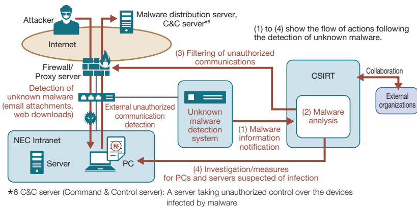
Detection of unknown malware and unauthorized communications
