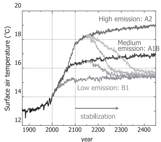
Fig. 2 Changes in globally averaged annual mean surface air temperature over time.
